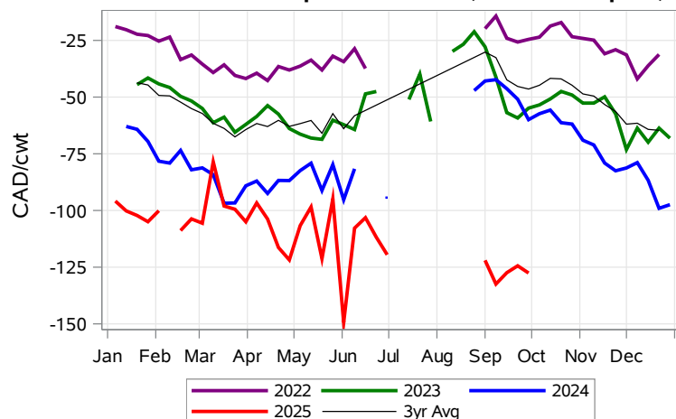
Feeder to Calf Spread Alberta (Week of Sep 29)
