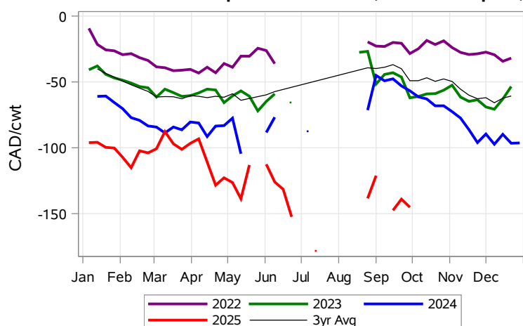
Feeder to Calf Spread SaskMan (Week of Sep 29)
