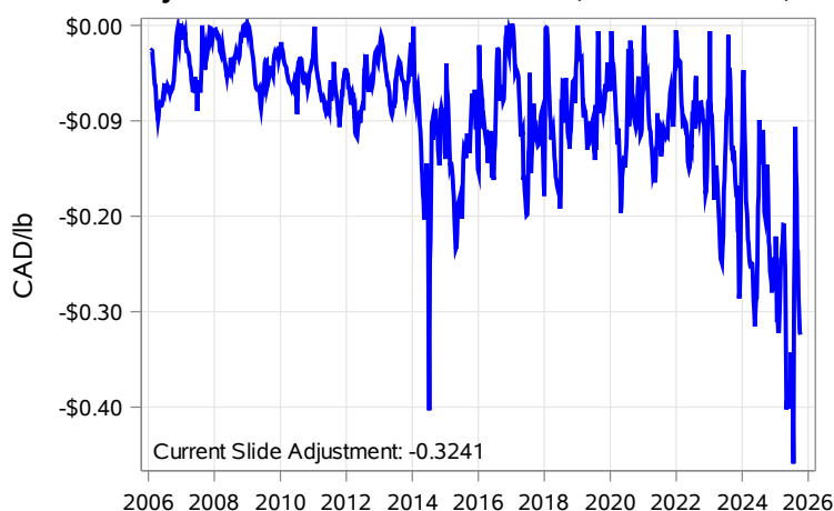
Slide Adjustment 750-950lbs Alberta (Week of Oct 6)
